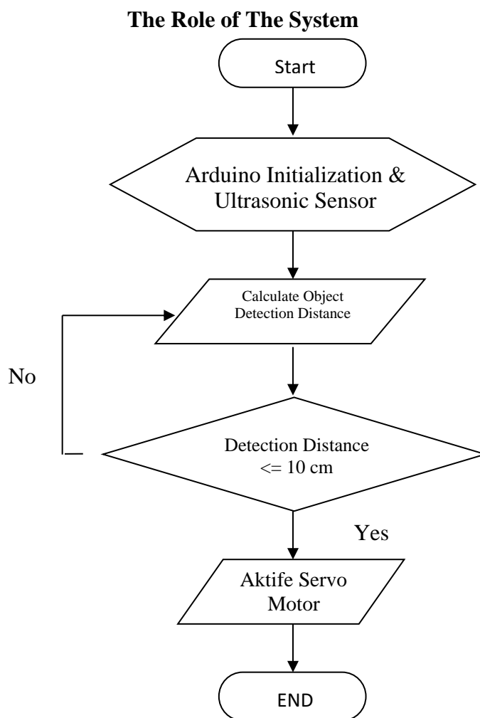
Figure 5. System Flowchart
